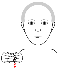
b. SOSED
