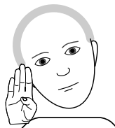
c. FANT
