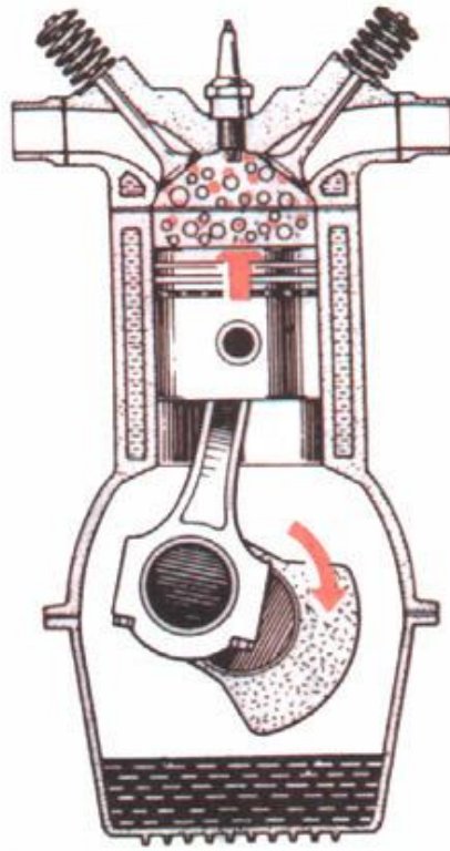
Compression
